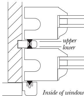
The position of the nylon seals in a refurbished box sash
