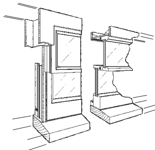
Sliding sashes with SASHSEAL™ draught control system and sealed unit double glazing (viewed from outside)
